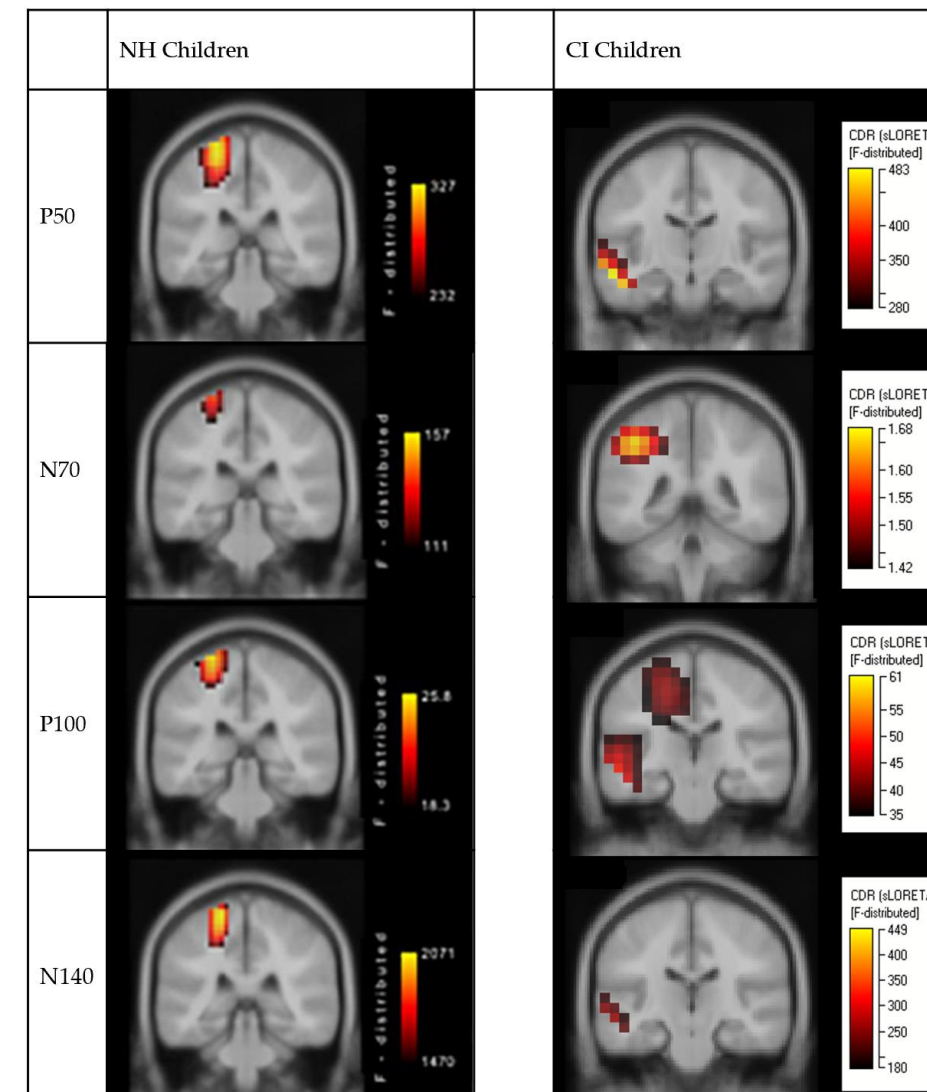
Figure 2. CDR images illustrating cortical activation underlying CSEP peak components P50, N70, P100, and N140 on coronal MRI slices in NH children (left panel; n=35, age range 5.84-17.27 years, mean age 10.54) [4] and in children with CIs (n=10; right panel)
