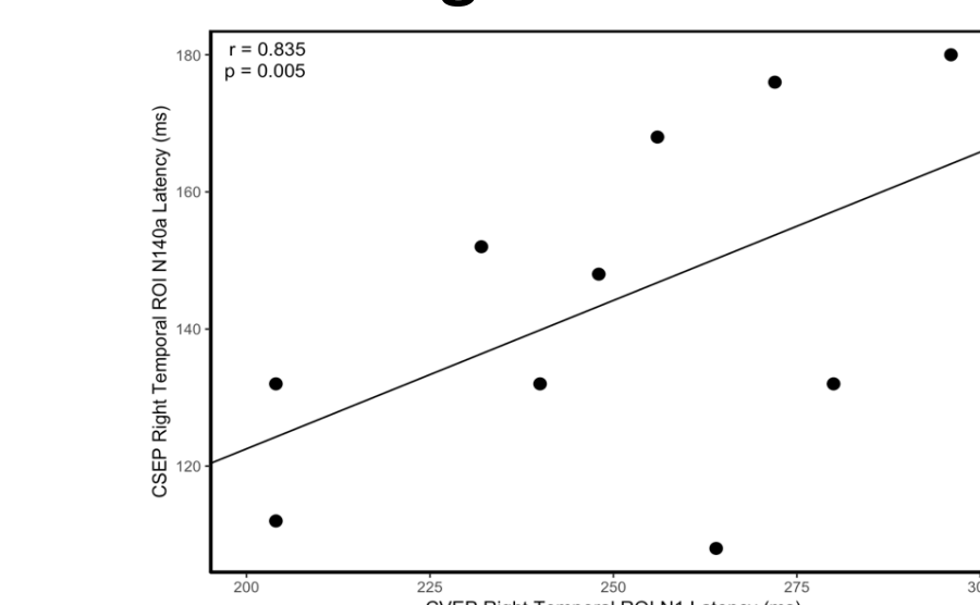
Figure 6. Scatter plot illustrating the correlation between CSEP 140a latency and CVEP N1 latency in the right temporal ROI in children with CIs (n=10)
