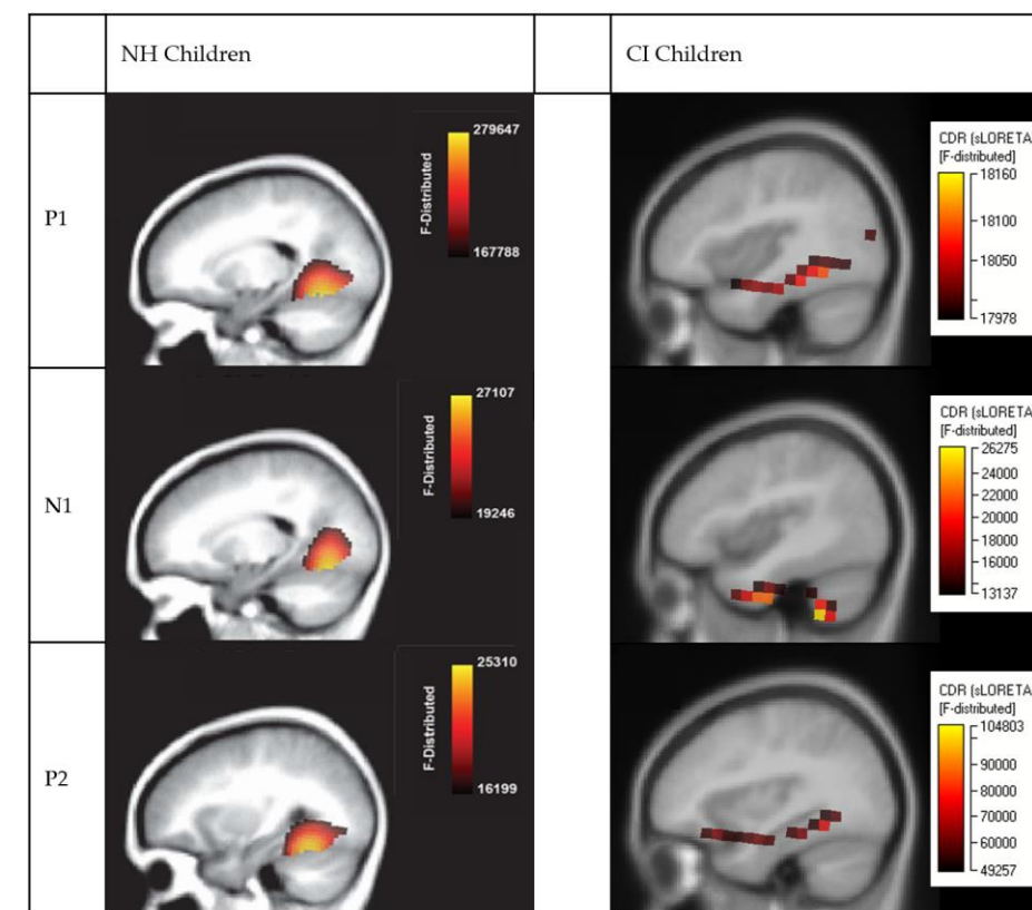
Figure 1. CDR images illustrating cortical activation underlying CVEP peak components P1, N1, and P2 on sagittal MRI slices in NH children (left panel; n=41, age range 5.87–14.53 years, mean age 10.32) [3] and in children with CIs (n=10; right panel)
